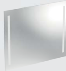
Illuminated mirror element , with integrated switch, T5, 2 x 24 W, 4000 K, 230 V, ~50 Hz, IP 44, safety class 2, energy class A, 800 x 650 x 36 mm, Model-no. 800480.
